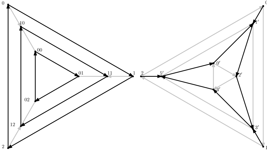
Figure 13.27: A plane representation of \text{Cay}(\mathbb{Z}_3^{[1]} \xrightarrow{f(1)=(0,1)} (\mathbb{Z}_2 \times \mathbb{Z}_3)^{(1,0)}) and \text{Cay}(\mathbb{Z}_3^{[1]} \xrightarrow{f(1)=2'} \mathbb{Z}_6^{[1']}) .
