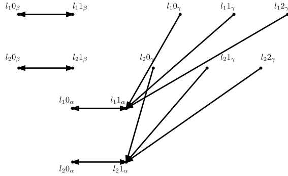
Diagram (b). \text{Cay}(S, \{(l_2), 1_\beta\})
