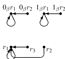
Diagram (c). \text{Cay}(S_\alpha \cup S_\beta, \{(0_\beta, r_1)\})
