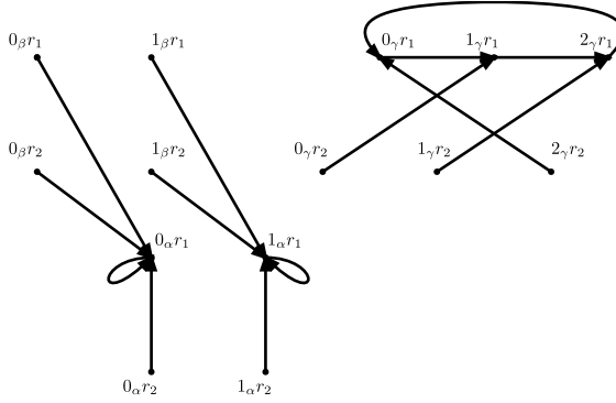
Diagram (c). \text{Cay}(S, \{(1_\gamma, r_1)\})
