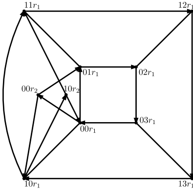
Figure 13.17: On the way to \text{Cay}(\mathbb{Z}_2 \times \mathbb{Z}_4 \times R_2, \{(1, 0, r_1), (0, 1, r_1), (0, 0, r_2)\}) .
