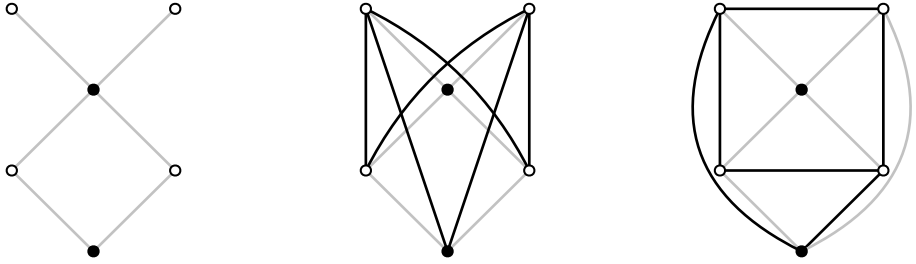
Figure 13.22: An X semilattice, with meet-irreducibles as unfilled vertices and its cover relations in bold gray. From the left to right, the Hasse diagram, the Cayley graph, and a plane embedding of the latter (right).
