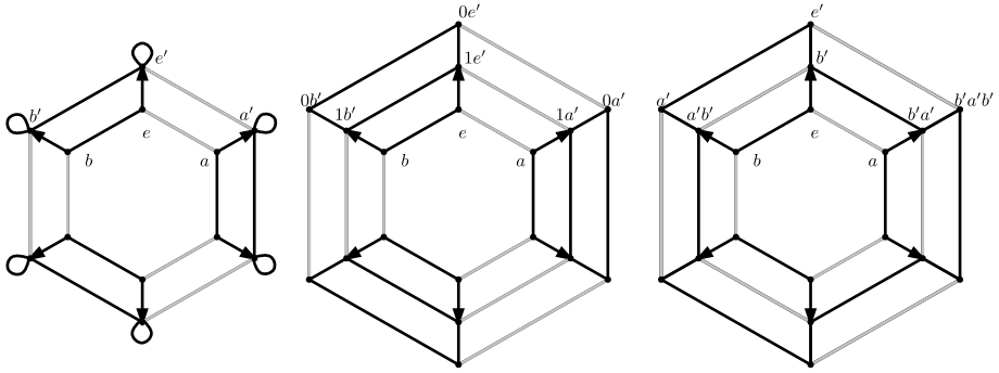
Figure 13.28: Several dihedral prisms: \text{Cay}(D_3^{\{a,b\}} \xrightarrow{f(a)=a', f(b)=(b')} D_3^{\{e'\}}) , \text{Cay}(D_3^{\{a,b\}} \xrightarrow{f(a)=(0,a'), f(b)=(0,b')} (\mathbb{Z}_2 \times D_3)^{\{(1,e')\}}) , \text{Cay}(D_3^{\{a,b\}} \xrightarrow{f(a)=a' b' a', f(b)=b'} D_6^{\{a'\}}) , (a' b' a' b')^2 = e' = e_{D_6} .
