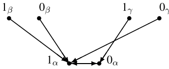
Diagram (f). \text{Cay}(S, \{1_\alpha\})
