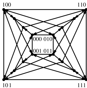
Figure 13.19: \text{Cay}(\mathbb{Z}_2 \times D_{2n} \times \mathbb{R}_2, \{(1, 1_{D_{2n}}, r_1), (0, a, r_2), (0, b, r_2)\}) .
