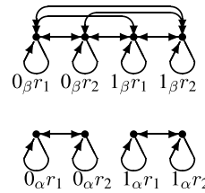
Diagram (b). \text{Cay}(S_\alpha \cup S_\beta, S_\beta)
