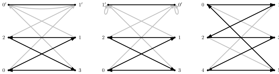
Figure 13.24: \text{Cay}(\mathbb{Z}_4^{\{1\}} \xrightarrow{f(1)=1'} \mathbb{Z}_2^{\{1'\}}) , \text{Cay}(\mathbb{Z}_4^{\{1\}} \xrightarrow{f(1)=1'} \mathbb{Z}_2^{\{0'\}}) , and \text{Cay}(\mathbb{Z}_6, \{1, 3\}) .
