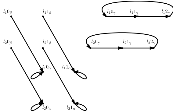
Diagram (c). \text{Cay}(S, \{(l_1), 1_\gamma\})
