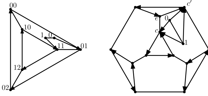
Figure 13.26: The plane Cayley graphs of \mathbb{Z}_2^{[1]} \xrightarrow{f(1)=(1,0)} \mathbb{Z}_2 \times \mathbb{Z}_3^{\{(0,1)\}} and the graph \text{Cay}(\mathbb{Z}_2^{[1]} \xrightarrow{c_e} A_4^{[c,c']}) .
