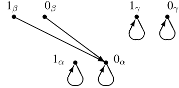
Diagram (e). \text{Cay}(S, \{0_\gamma\})
