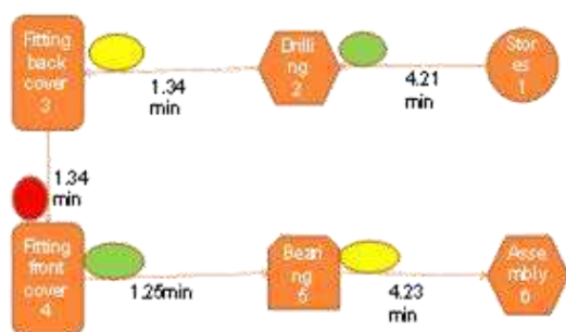
Fig. 3: Layout After
