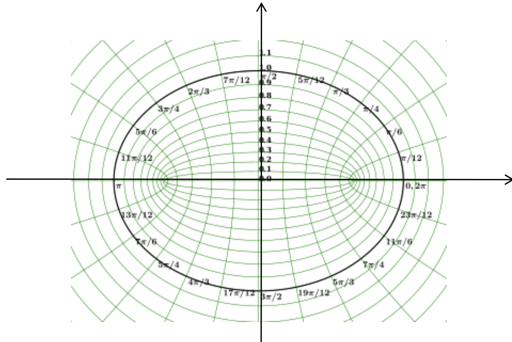
Elliptic coordinates
